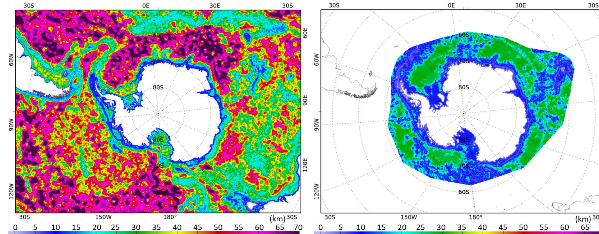
Fig. 2: Mesh resolution (km) of the FES2014 global model (left) and the ALBATROSS v1 regional model (right).
