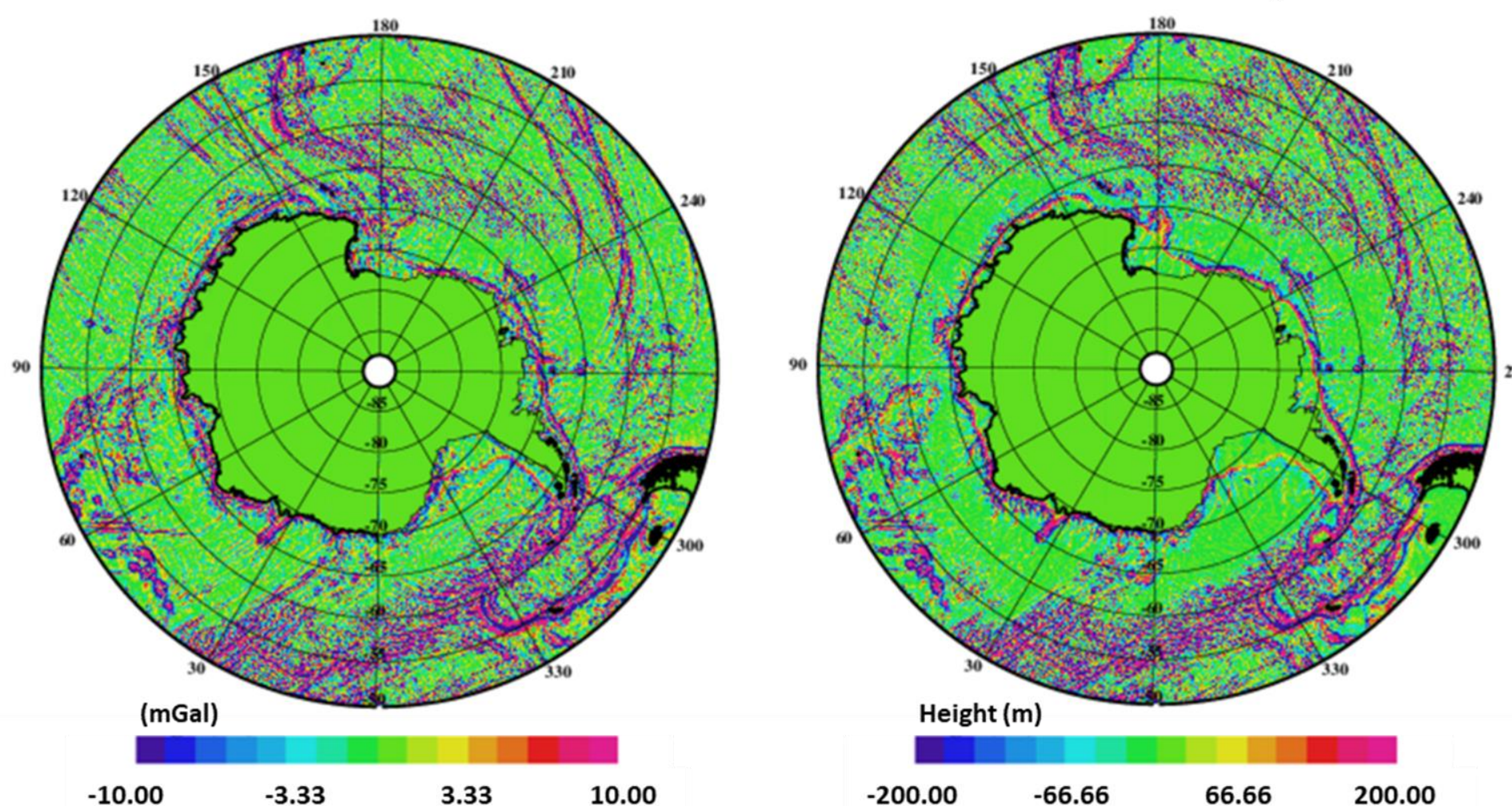
Fig. 5: DTU21 gravity field (left) and BedMachine+RTopo-2.0.4 bathymetry (right) band-pass filtered between 20 and 60 km.
