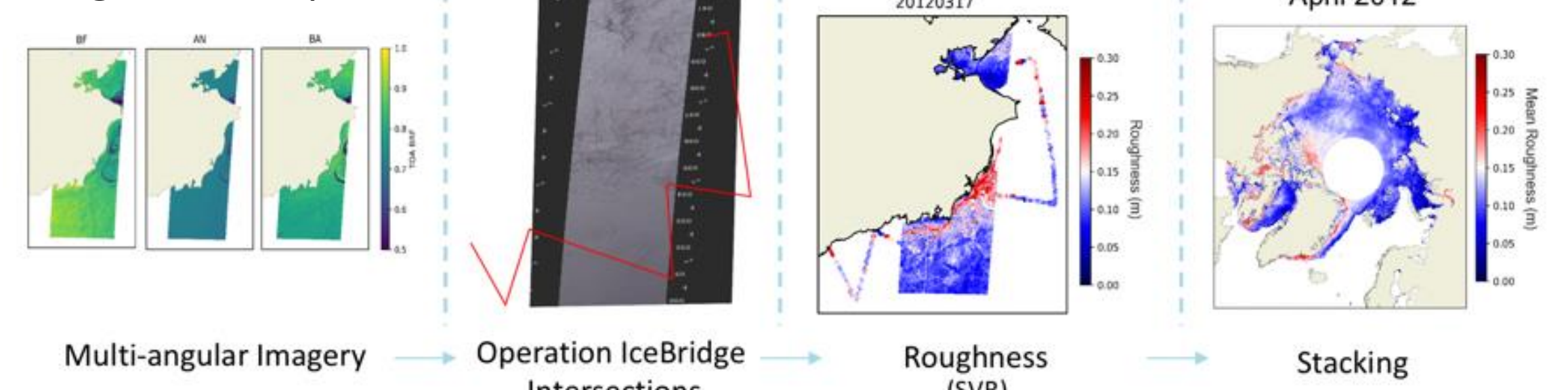
Fig. 6: Process diagram for the production of sea ice surface roughness maps from MISR
