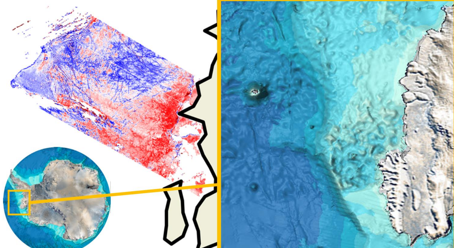
Fig. 7: MISR sea ice surface roughness (red to blue colors, left) and bathymetry features (right) close to the Antarctic Peninsula
