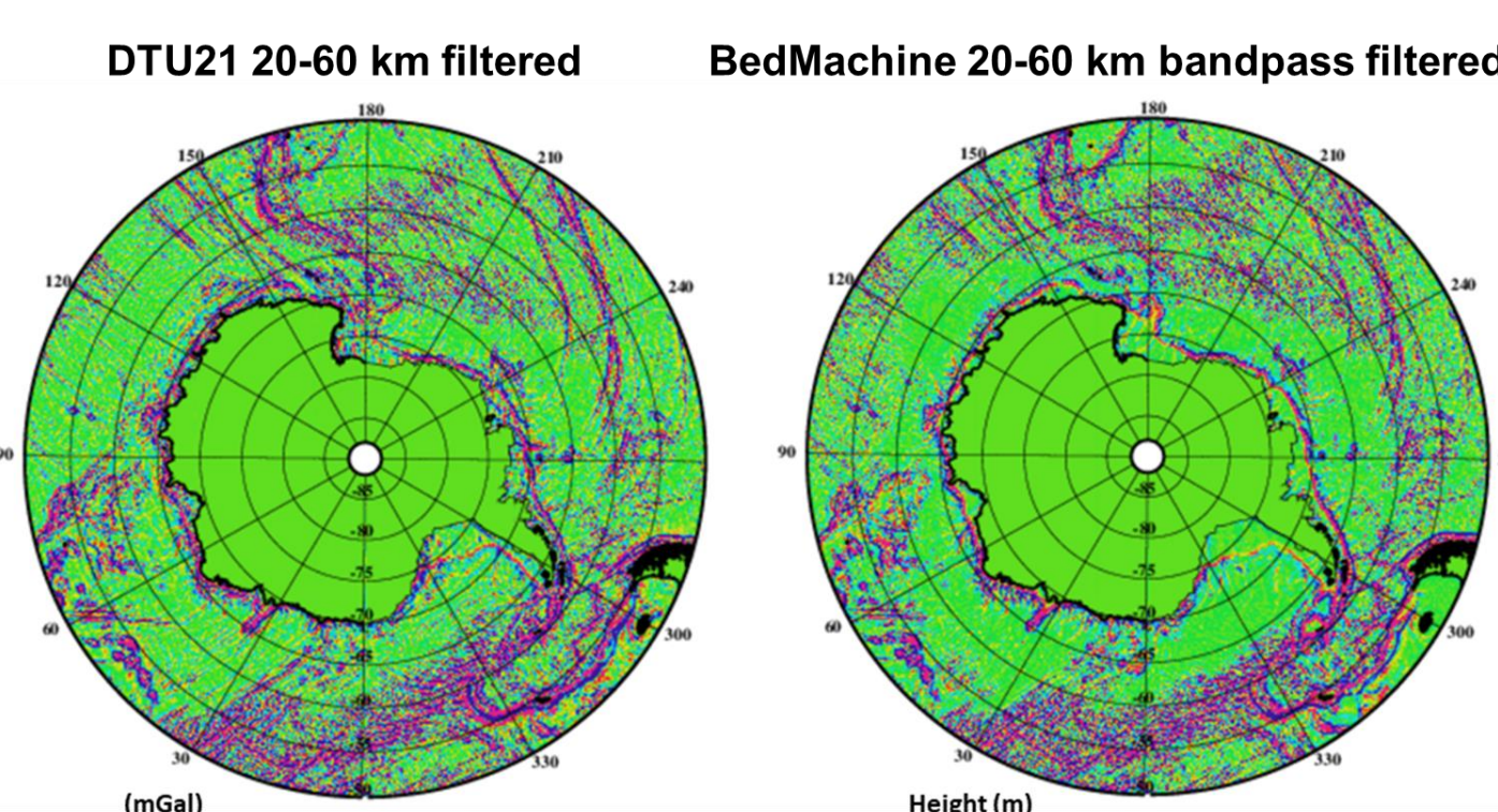
Fig. 3: DTU21 gravity field (left) and BedMachine+RTopo-2.0.4 bathymetry (right) band-pass filtered between 20 and 60 km.
